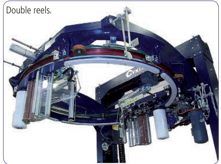
External pre-stretch dry system.
